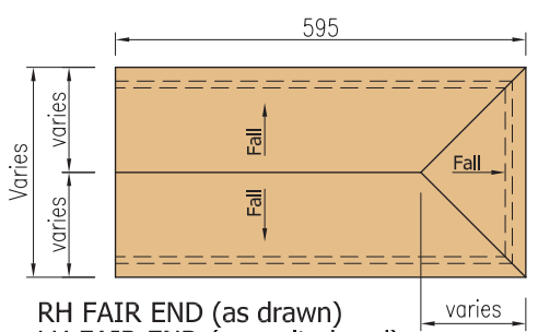
Coping type CP2
