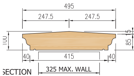
Section type CP3C Weight = 85kgs/lm
