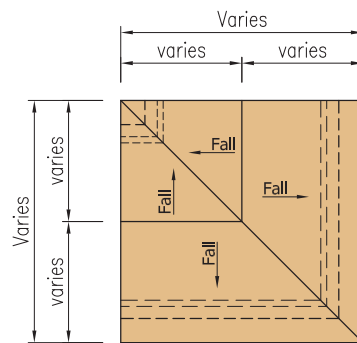
90° RETURN 90° return available to all section types.
