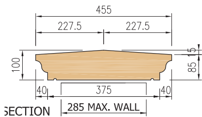
Section type CP3B Weight = 78kgs/lm
