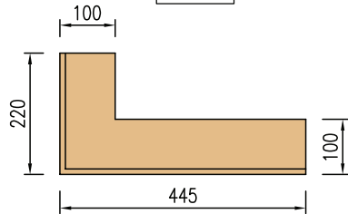
PLAN RA4/RA5
