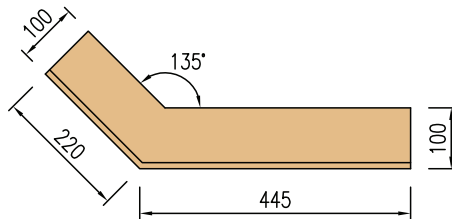
PLAN RA8/RA9
